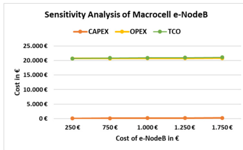
Figure 6. SA of Macrocell CAPEX, OPEX, and TCO in relation to the eNB
