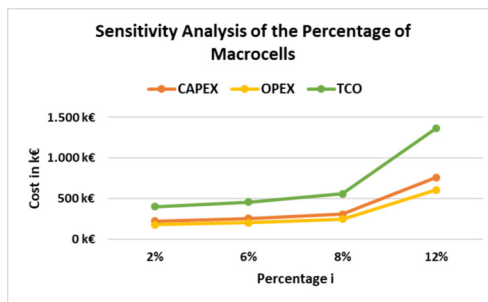
Figure 15. Macrocells vs. small cells SA of MacroCell CAPEX, OPEX, and TCO in relation to the i
