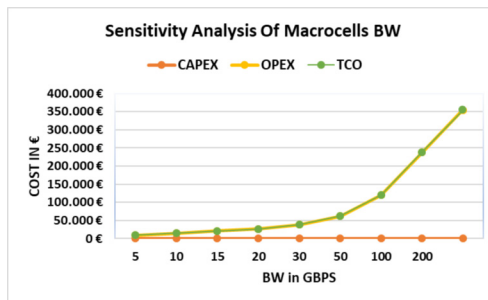
Figure 9. Macrocells vs. small cells: SA of Macrocell CAPEX, OPEX, and TCO in relation to the BW
