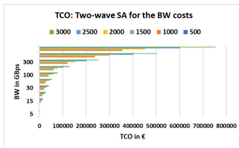
Figure 21. Two-way SA of Macrocell in relation to the f_{BW} and BW -TCO
