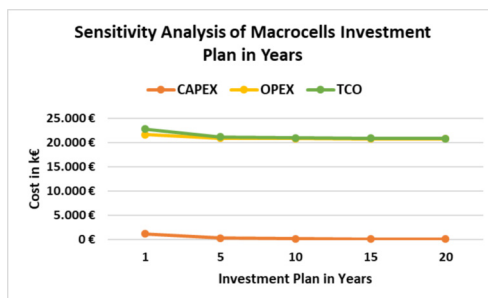
Figure 17. Macrocells vs. small cells SA of MacroCell CAPEX, OPEX, and TCO in relation to the years of investment n
