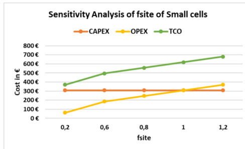
Figure 14. Macrocells vs. small cells SA of small cell CAPEX, OPEX, and TCO in relation to the f_{st}
