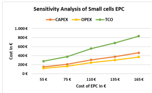
Figure 8. Macrocells vs. small cells: SA of small cell CAPEX, OPEX, and TCO in relation to the EPC
