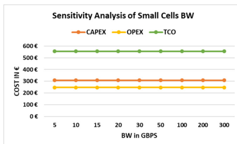
Figure 10. SA of small cells CAPEX, OPEX, and TCO in relation to the BW
